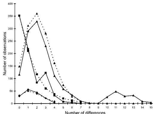
FIGURE 3. Mismatch distributions for clade A (triangles) showing a unimodal pattern consistent with population growth, clade B (diamonds) showing a unimodal pattern consistent with population growth, and Baja samples (clade C, squares) combined showing a unimodal pattern consistent with population growth. For each distribution, the expectation for a population that has recently expanded is shown with a dashed line.
