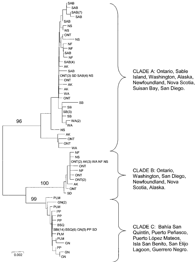
FIGURE 2. Neighbor-joining tree of haplotypes (based on pairwise distances) showing three major groups (the same topology was recovered in maximum parsimony analyses). Numbers above branches are percentage of bootstrap replicates supporting that node. No other nodes received greater than 60% support. Sampling locations are identified as follows: SAB = Sable Island, NS = Nova Scotia, ONT = Ontario, NF = Newfoundland, AK = Alaska, SD = San Diego, WA = Washington, SB = Suisan Bay, PLM = Puerto López Mateo, GN = Guerrero Negro, PP = Puerto Peñasco, BSQ = Bahía San Quintín, and SBI = Isla San Benito. Numbers in parentheses indicate numbers of individuals with that haplotype.
